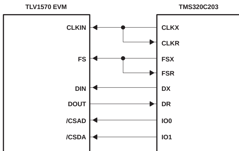
Figure 4–1. Example Hookup With TMS320C203 DSP
